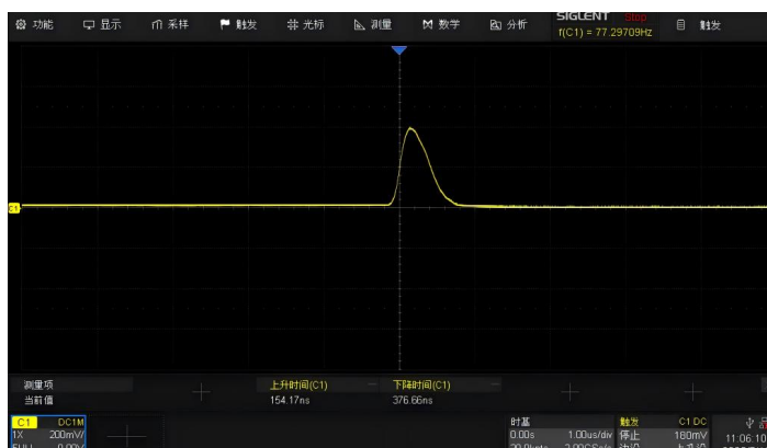
Output signal waveform,the oscilloscope input impedance 1MΩ
