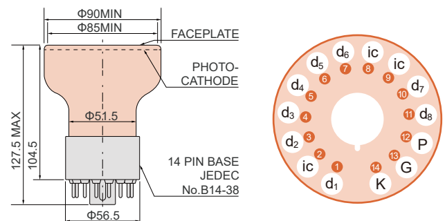
14-pins JEDEC connector (standard pin layout)
