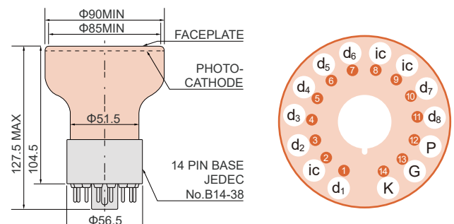
14-pins JEDEC connector (standard pin layout)
