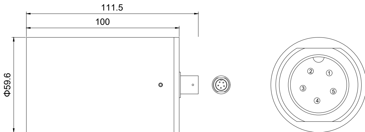
Unit: mm 2inch detector
