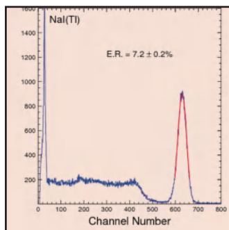
Energy resolution curve
