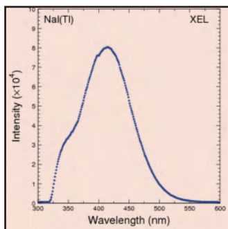
X-Ray excited Luminescence curve
