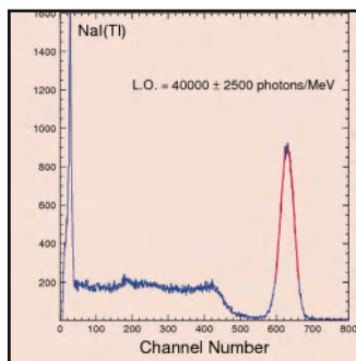
Light output curve
